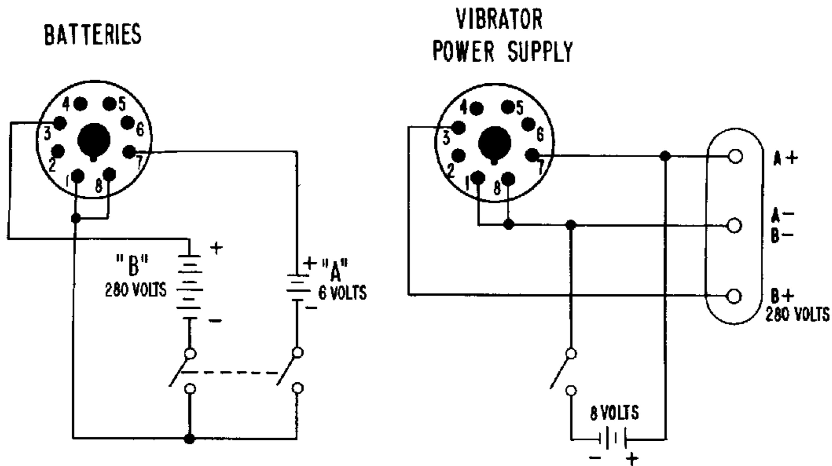
Fig. 5. Wiring Diagram for DC Operation
