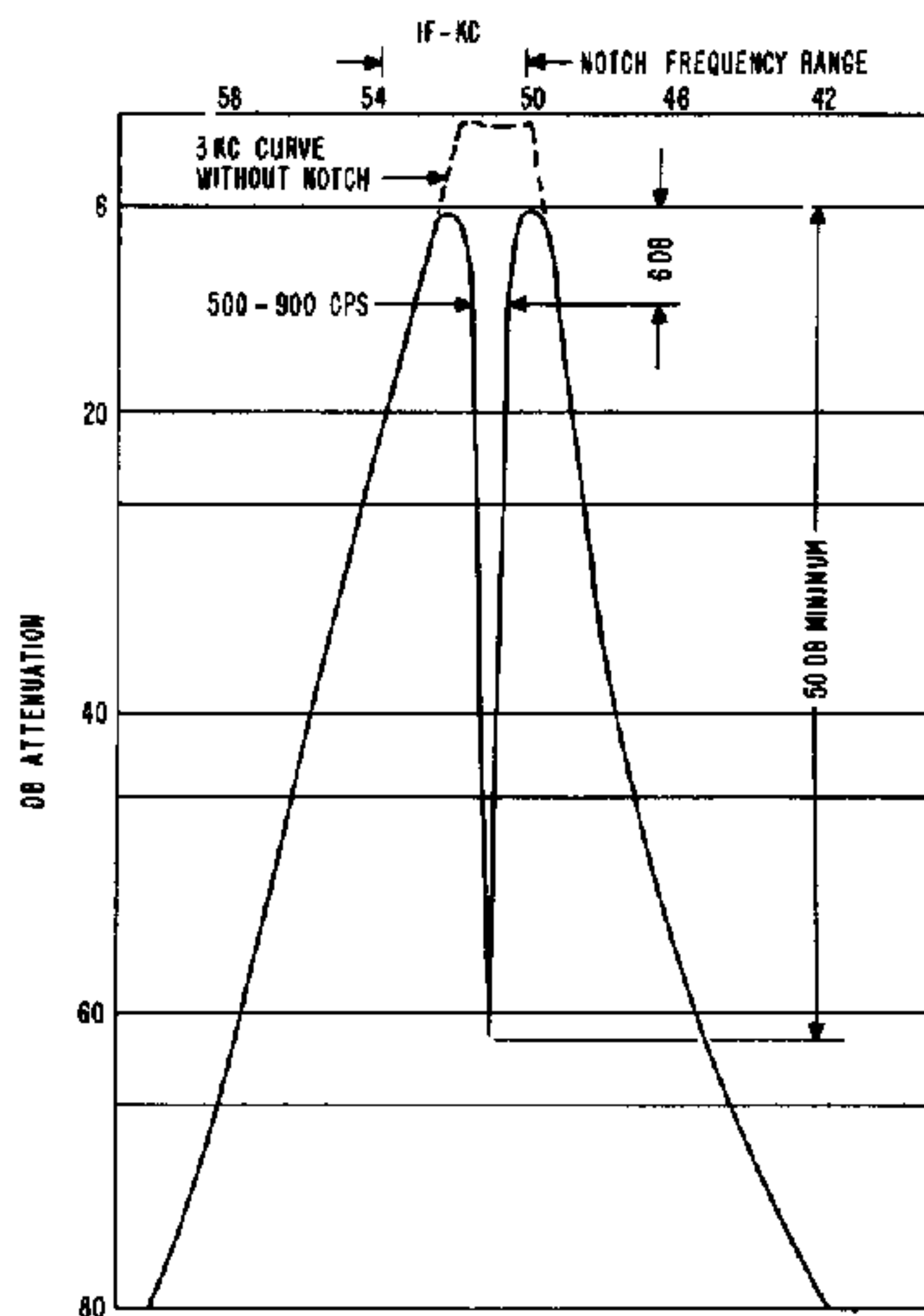
Fig. 9. IF Selectivity Curve with Notch
