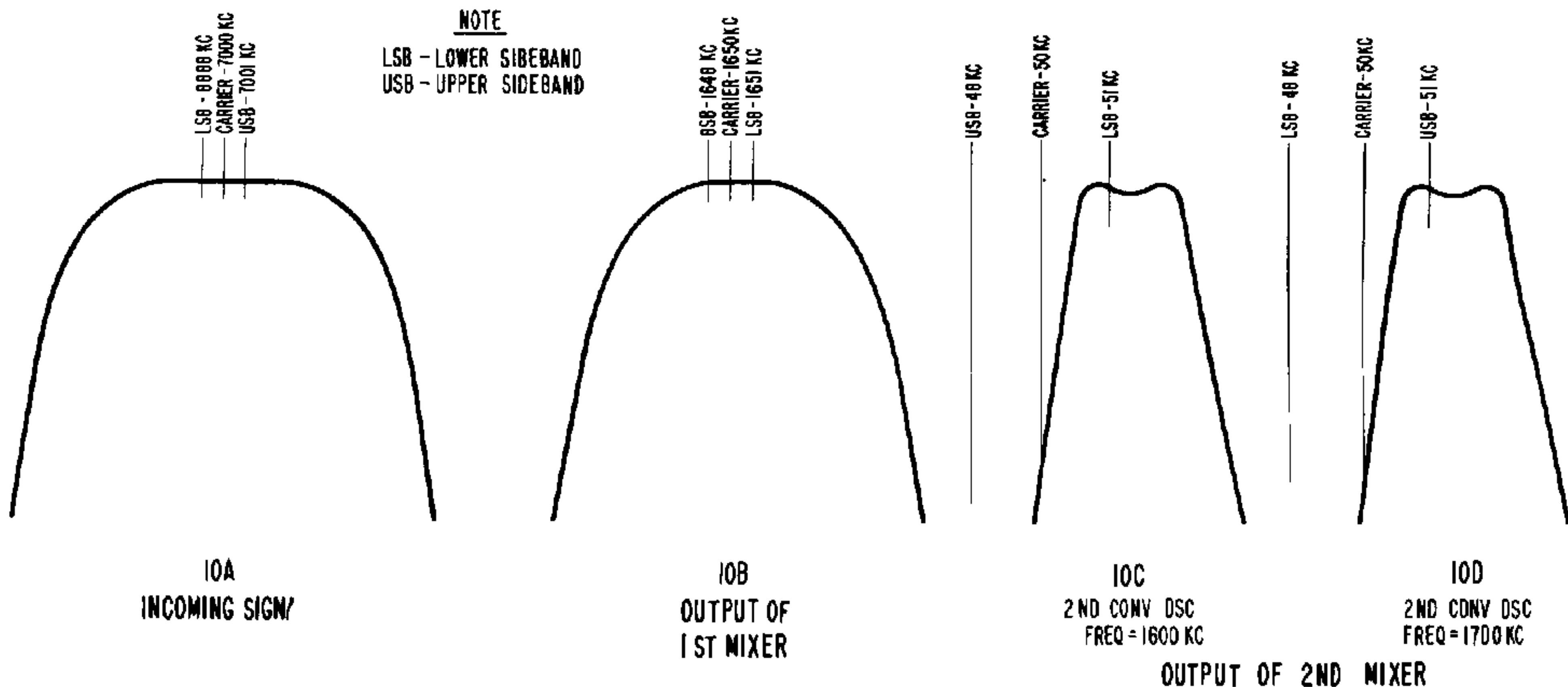
Fig. 10. Selectable-Sideband Response Curves
