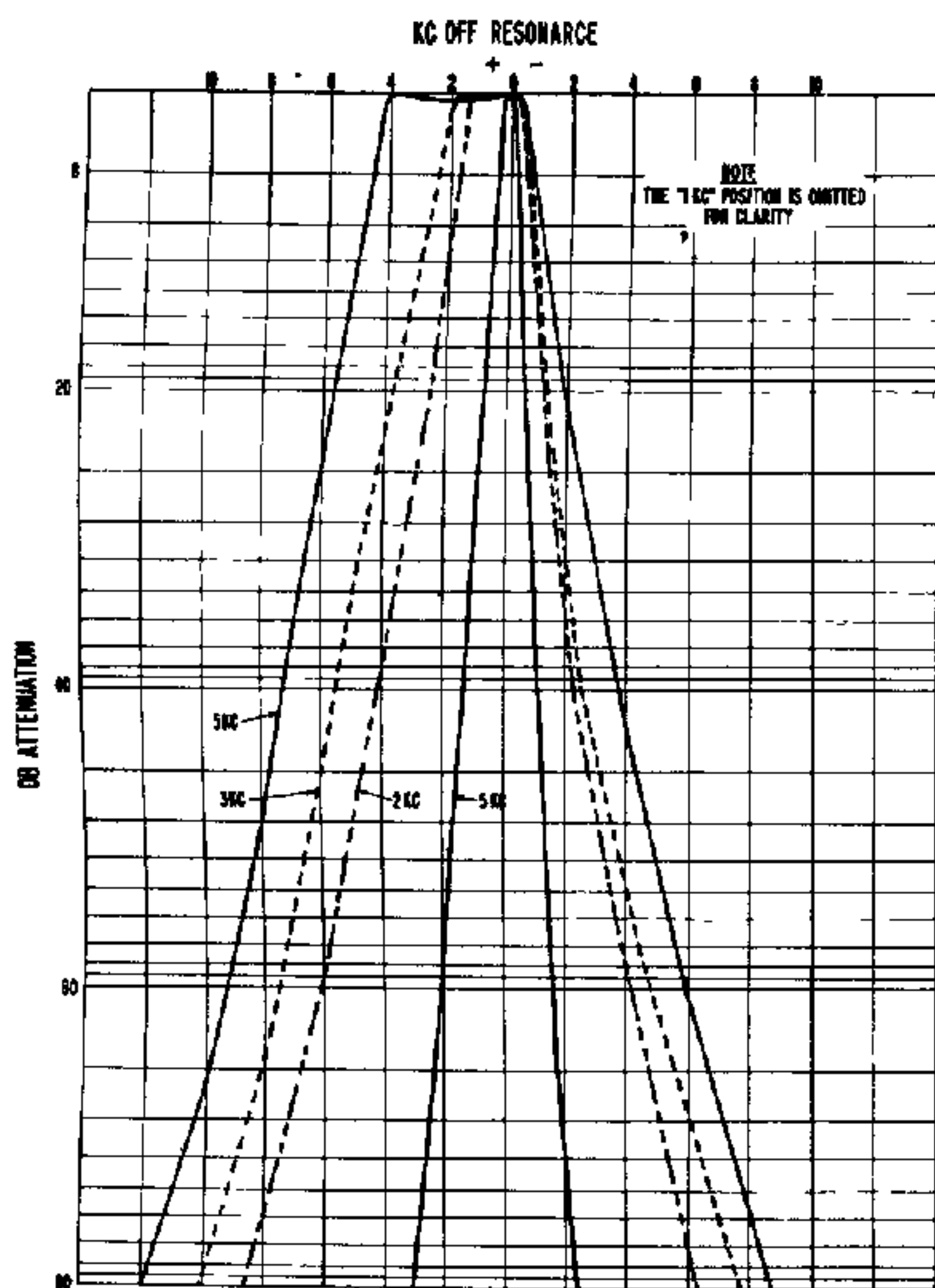
Fig. 8. IF Selectivity Curves
