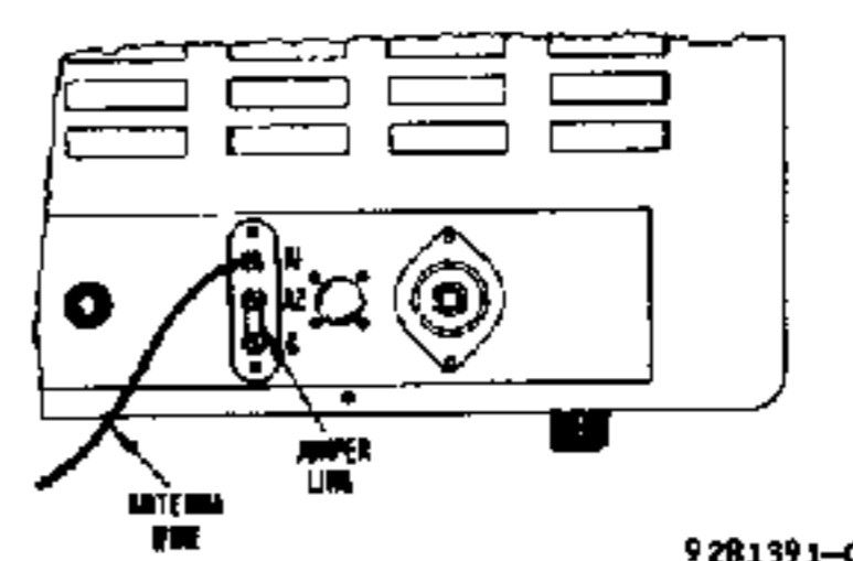
Fig. 2. Single Wire Antenna
