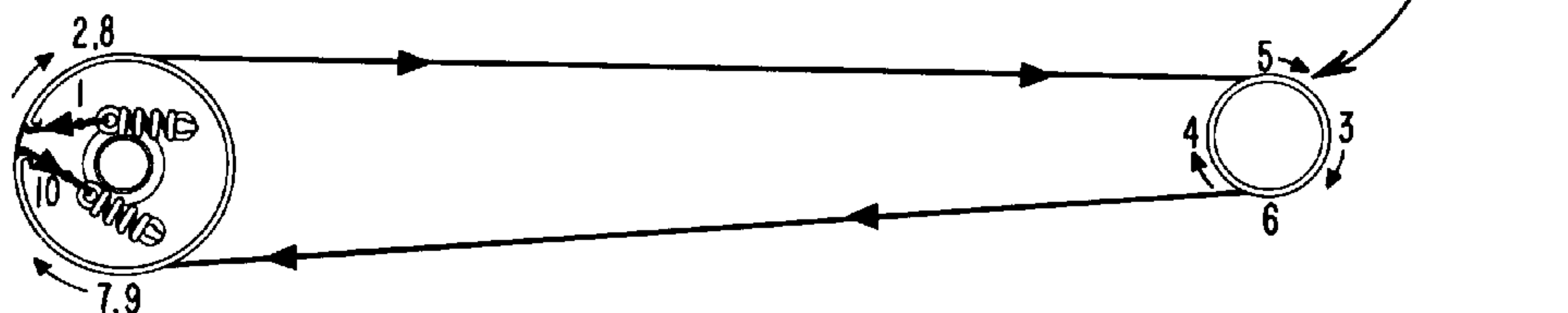
Fig. 14. Dial Cord Stringing Diagram
