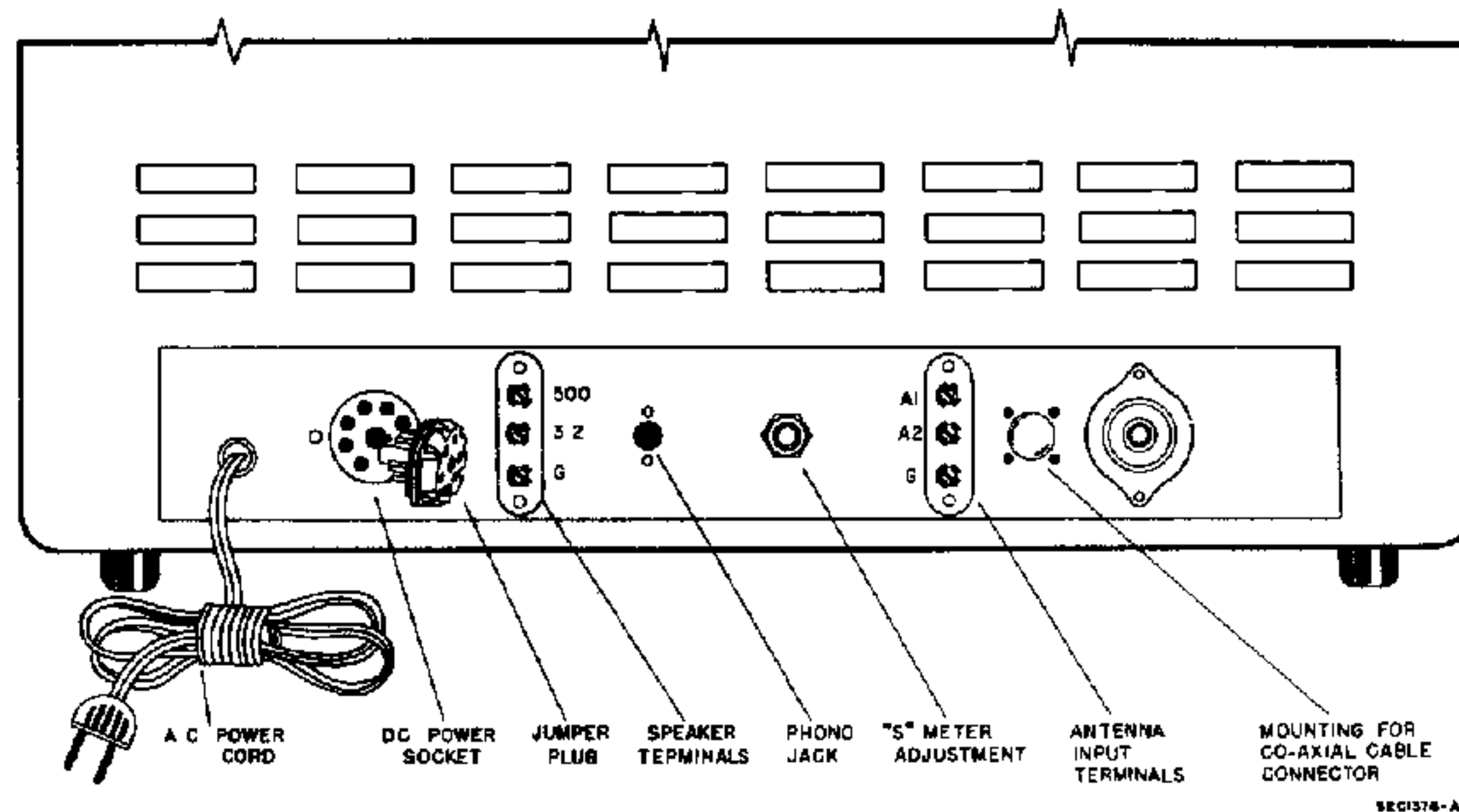
Fig. 4. Rear View of Receiver
