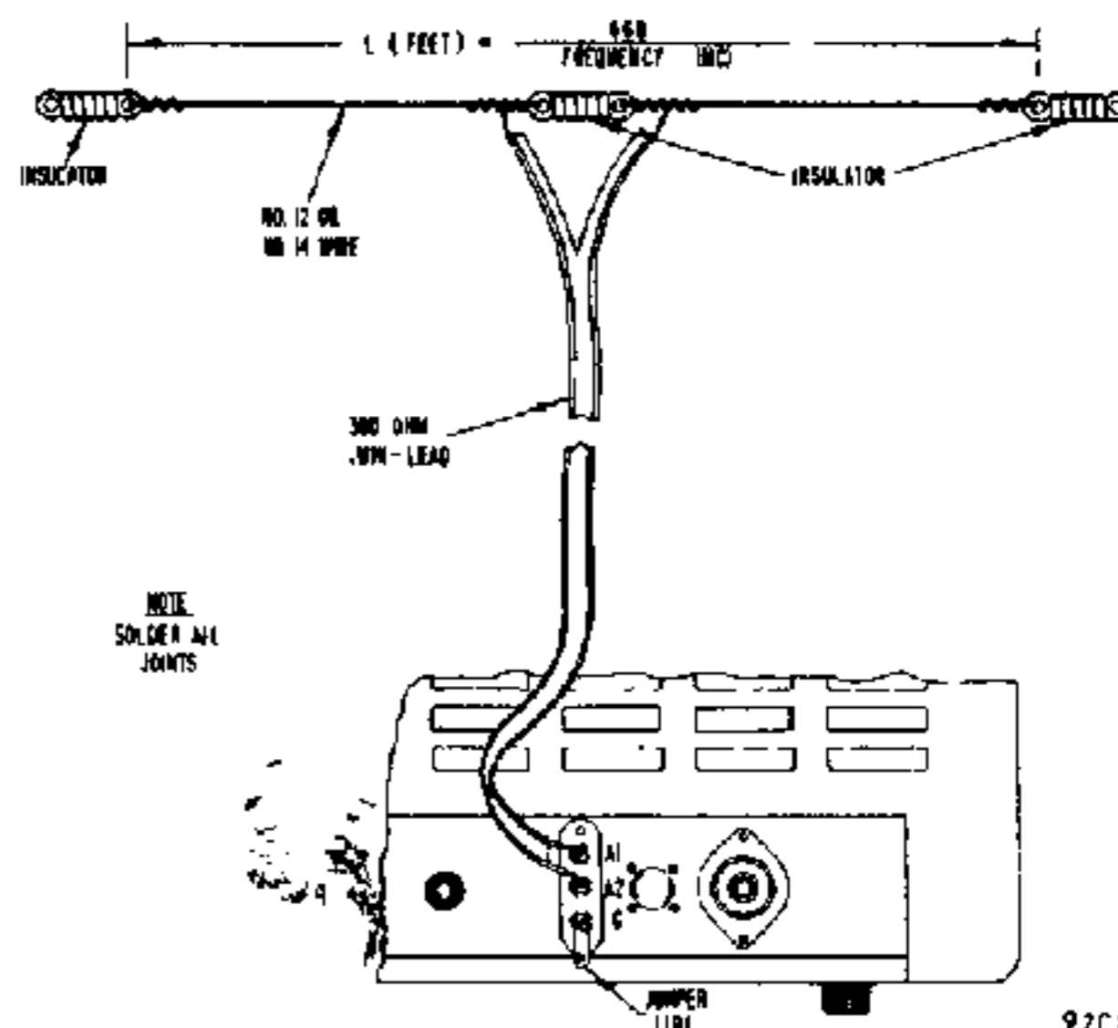
Fig. 3. Doublet Antenna Using Twin-Lead Transmission Line
