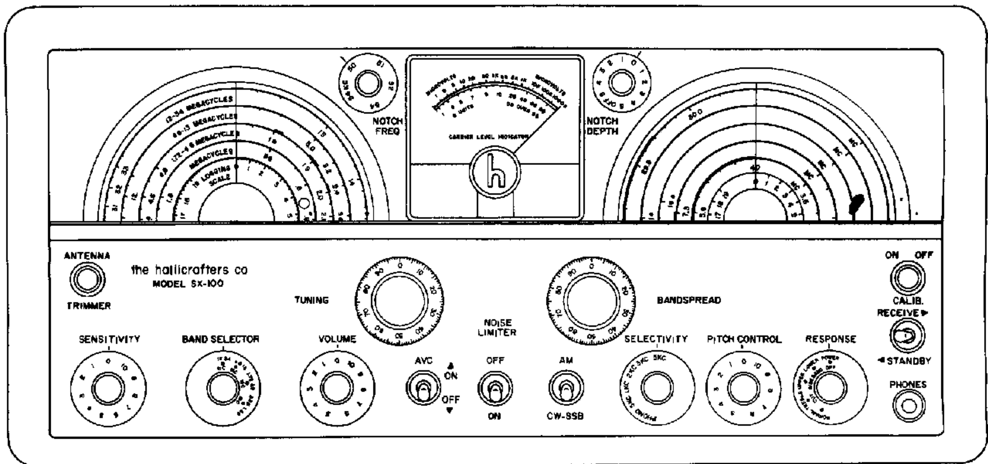
Fig. 7. Operating Controls
