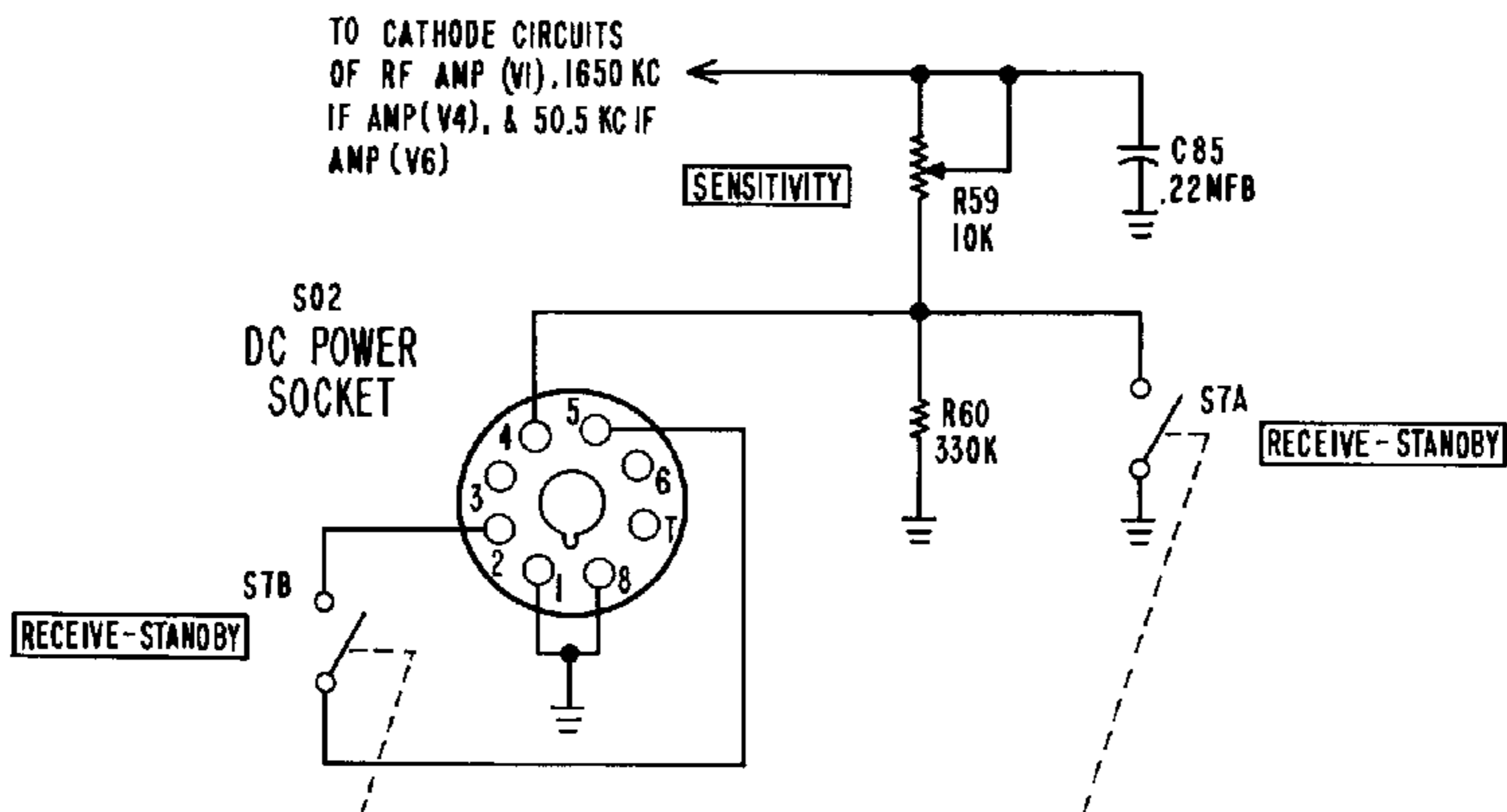
Fig. 6. Schematic Diagram of Sensitivity and Receive-Standby Circuits
